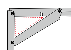
Robot Framework
